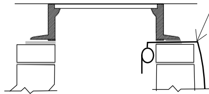
SECTION MH FRAME, COVER, GRADE RINGS WITH TRACER WIRE
